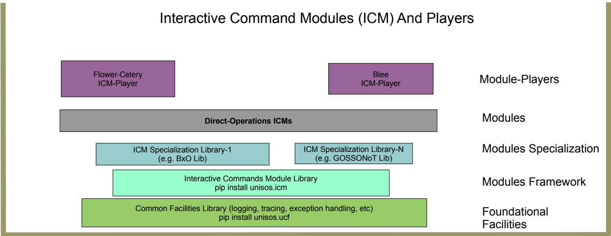
Figure 1: ICM Framework, Modules And Players
