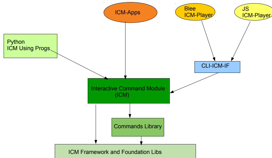
Figure 2: Direct Operations Interactive Command Modules (DO-ICM)
