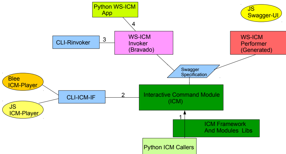
Figure 3: Web Services Interactive Command Module (WS-ICM) Using Swagger Code Generators
